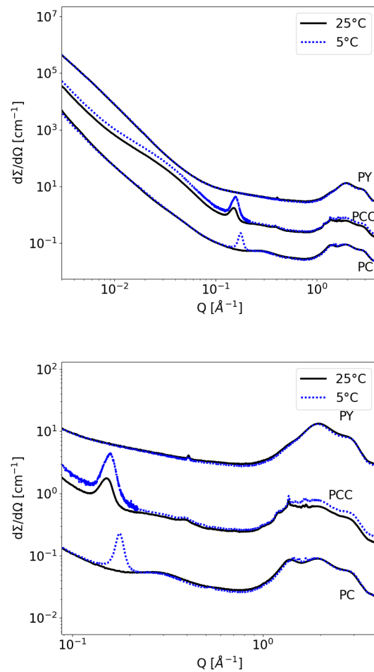
Top: Small Angle X-ray Scattering over a broad q-range, and zoomed into the high-Q-area. From top to bottom PY, PCC, PC, measured at 25 °C and 5 °C.
