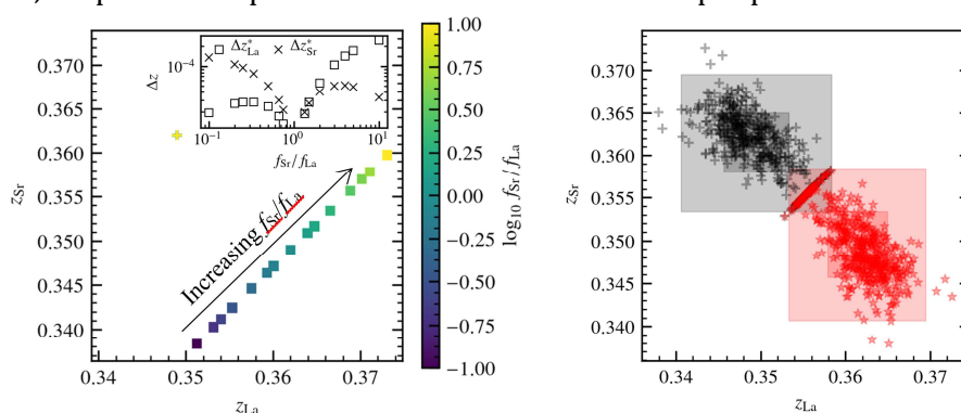
Figure 1. Left: PSC model study of the real (z_{\text{La}}, z_{\text{Sr}}) = (0.362, 0.349) and pseudosymmetric structure solution (z_{\text{La}}^*, z_{\text{Sr}}^*) as a function of La/Sr scattering strength. Inset: Respective variance \Delta z_{\text{La}, \text{Sr}} . The real solution shows no variance. Right: Monte-Carlo-Study of the structure solution including the single (2.3-times) trust region for random <20% intensity errors and equal scatterers.
